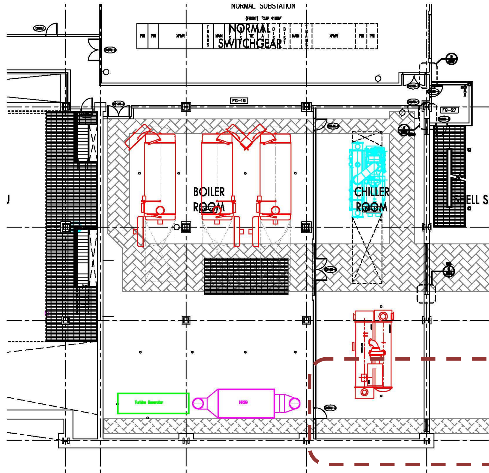
Figure 1: Alternate Design Boiler Room Layout Scale: 1/16" = 1'-0"
